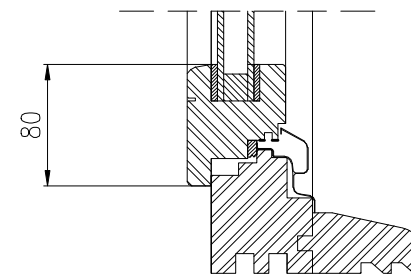
DETAIL B 1:5
