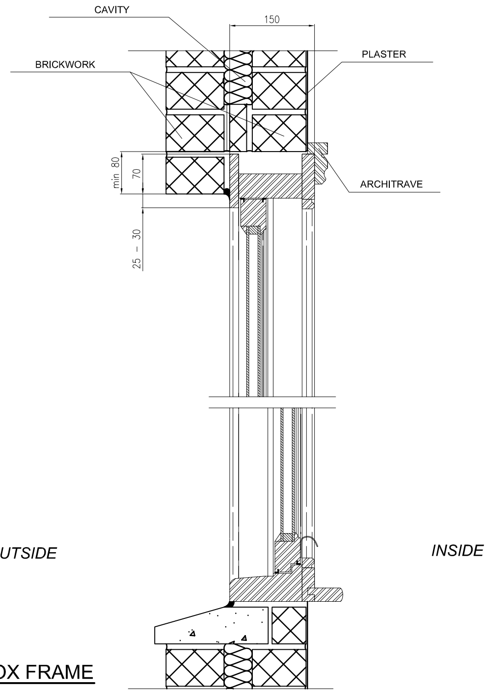
VERTICAL SECTION
